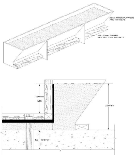
Fig.2 : Typical hopper system
