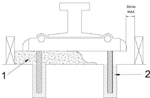
Fig.1: Typical detail of stanchion base plate
